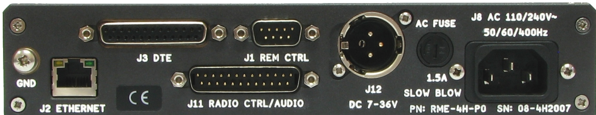
Fig2: Rear panel of the RM4 Unit
