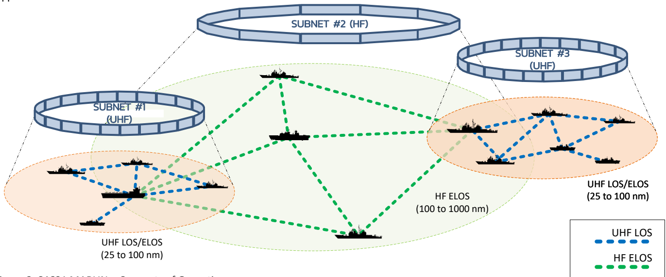
Figure 2: S4691 MARLIN – Concepts of Operation
